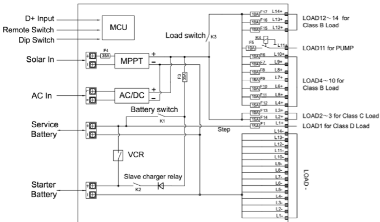
Figure 2 System Schematic
