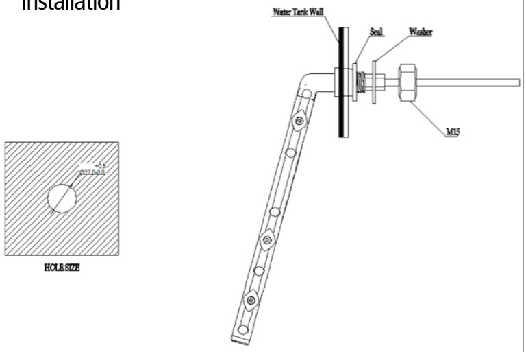
Figure 16 Installation of PMWS200
