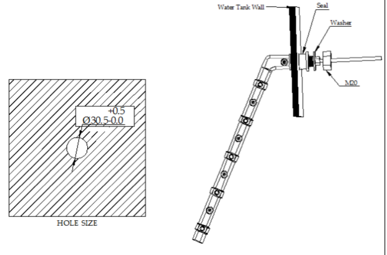
Figure 14 Installation of PMWS400
