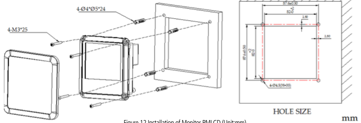
Figure 12 Installation of Monitor PMLCD (Unit:mm)
